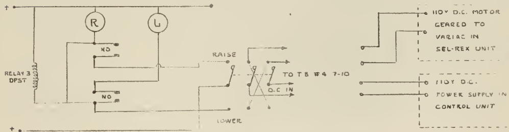
d. Arc Control Panel - Power raise-lower
